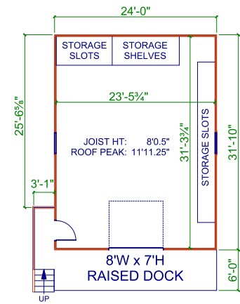
ELEVATED STORAGE SHED
