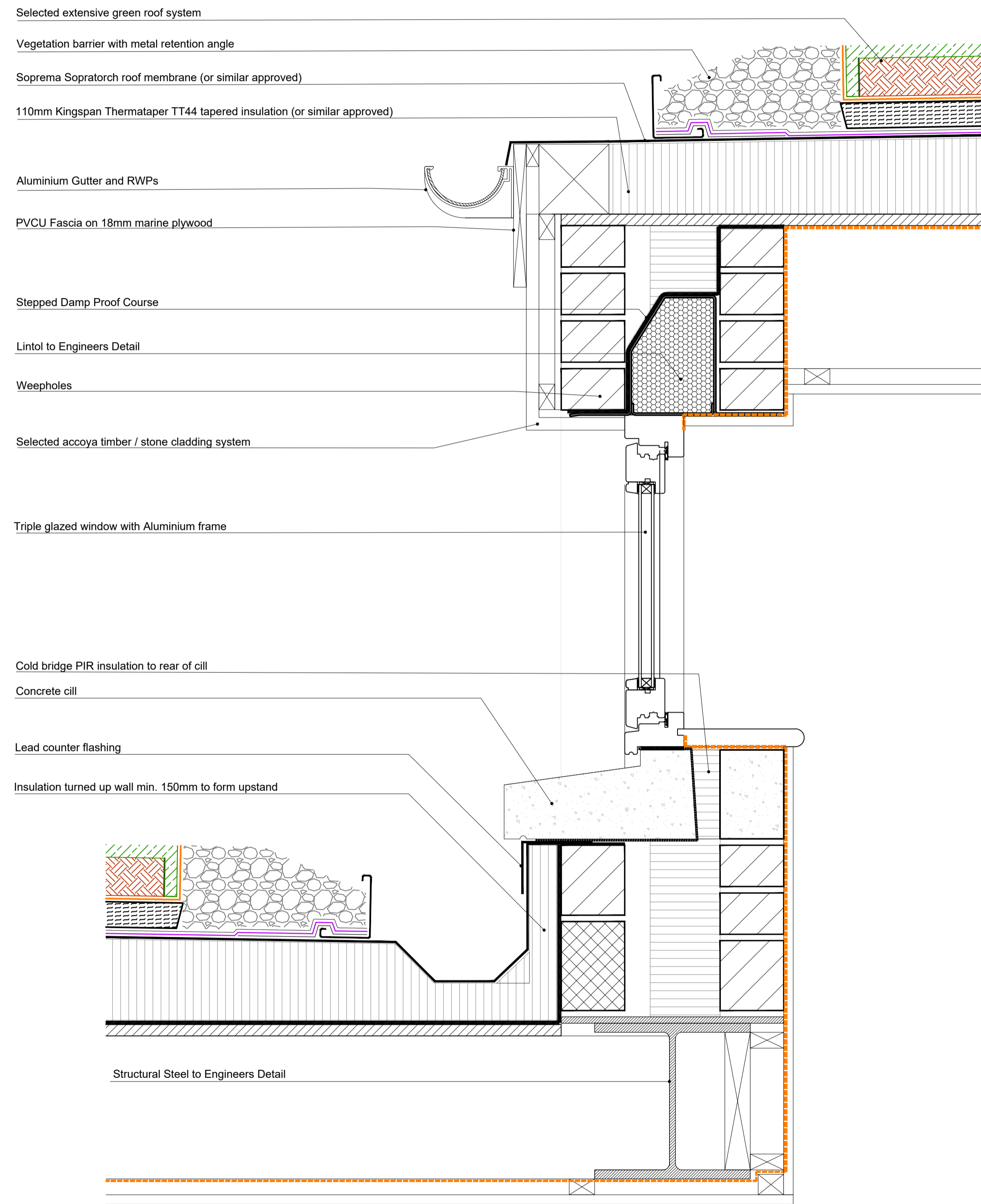
SECTION DETAIL 6 SCALE 1:5
