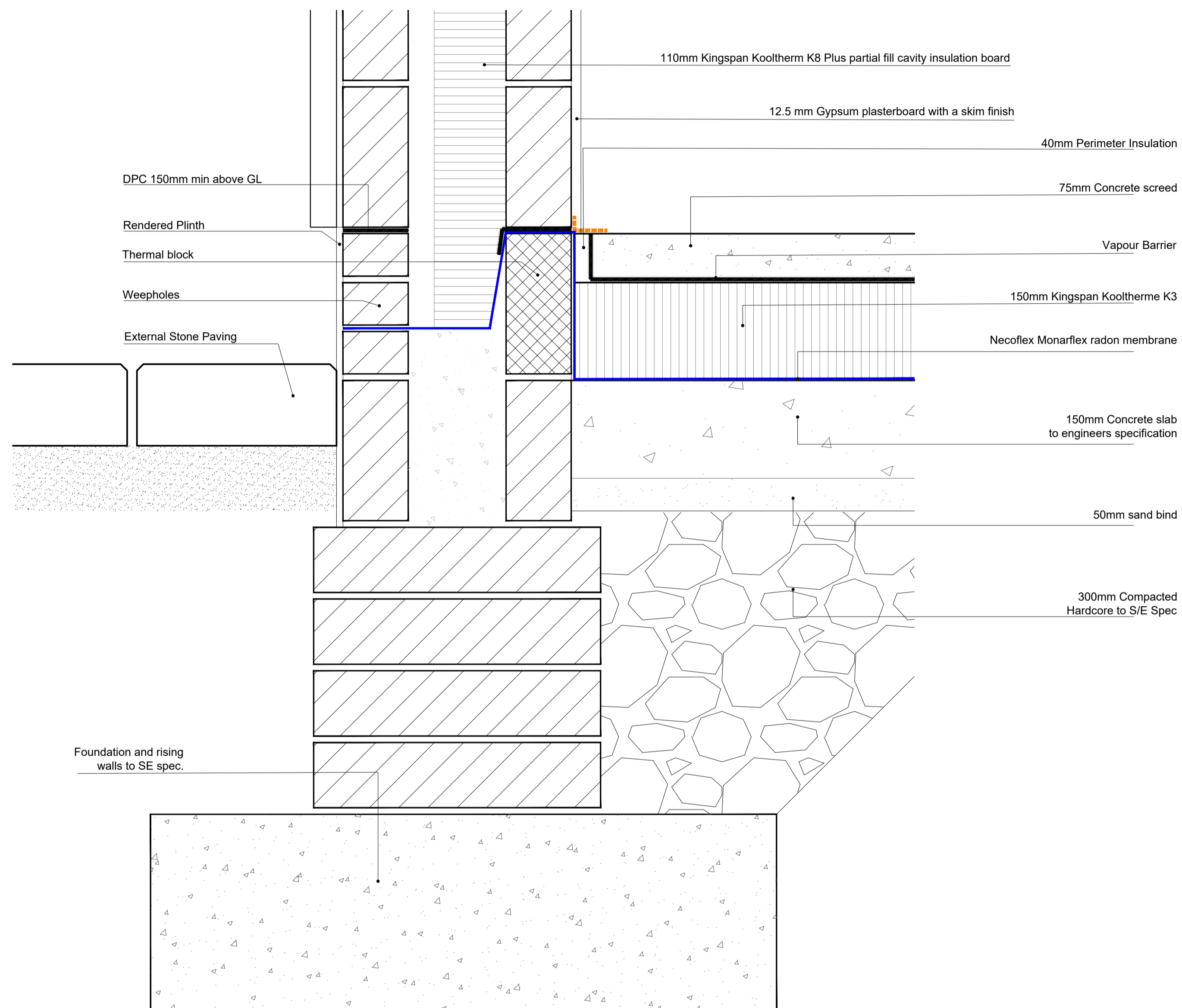
SECTION DETAIL 1 SCALE 1:5
