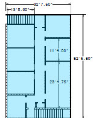
Second Floor Office Space
