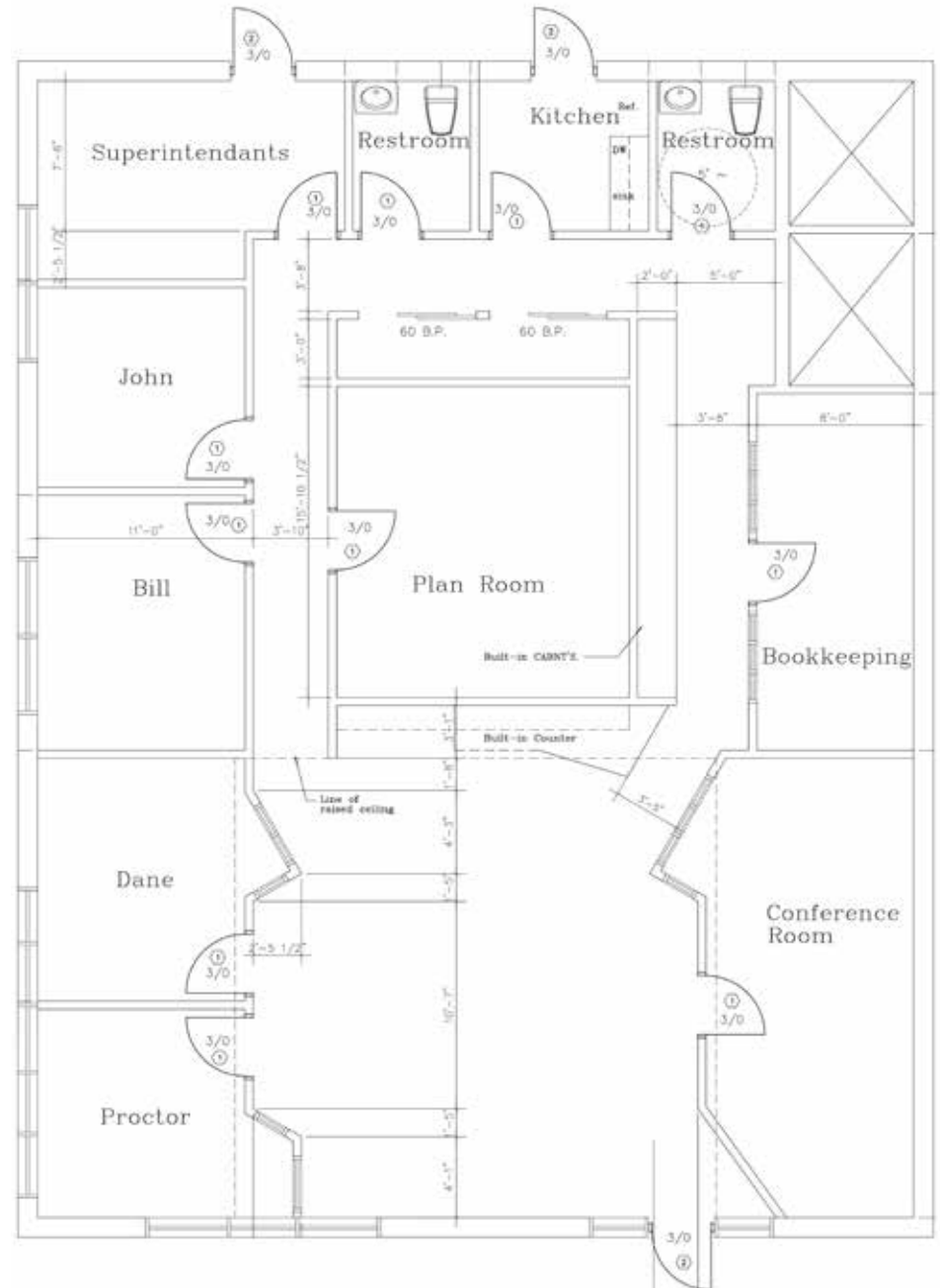
Suite 60/70 Floor Plan - 2,620 SF
