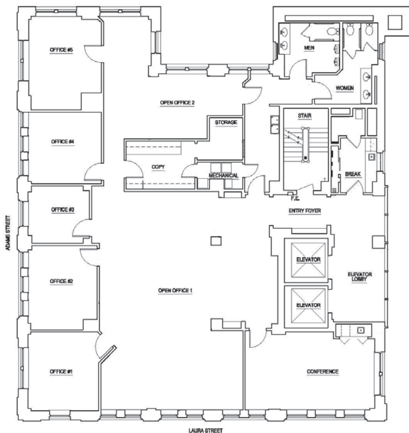
GREENLEAF BUILDING - TWELFTH FLOOR PLAN KENNETH SMITH ARCHITECTS, INC. 10-10-2015
