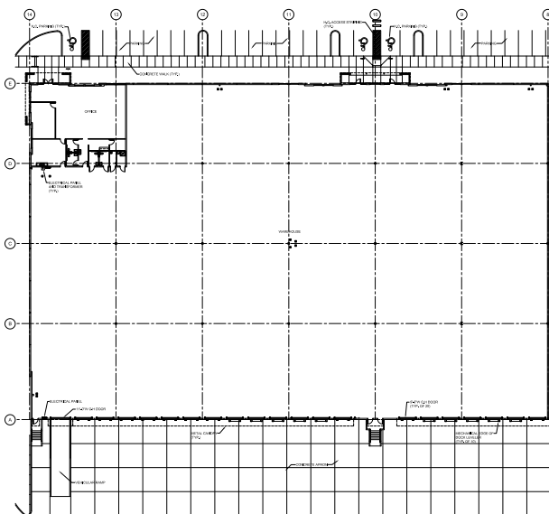
OVERALL AREA PLAN - 68,289 SF
