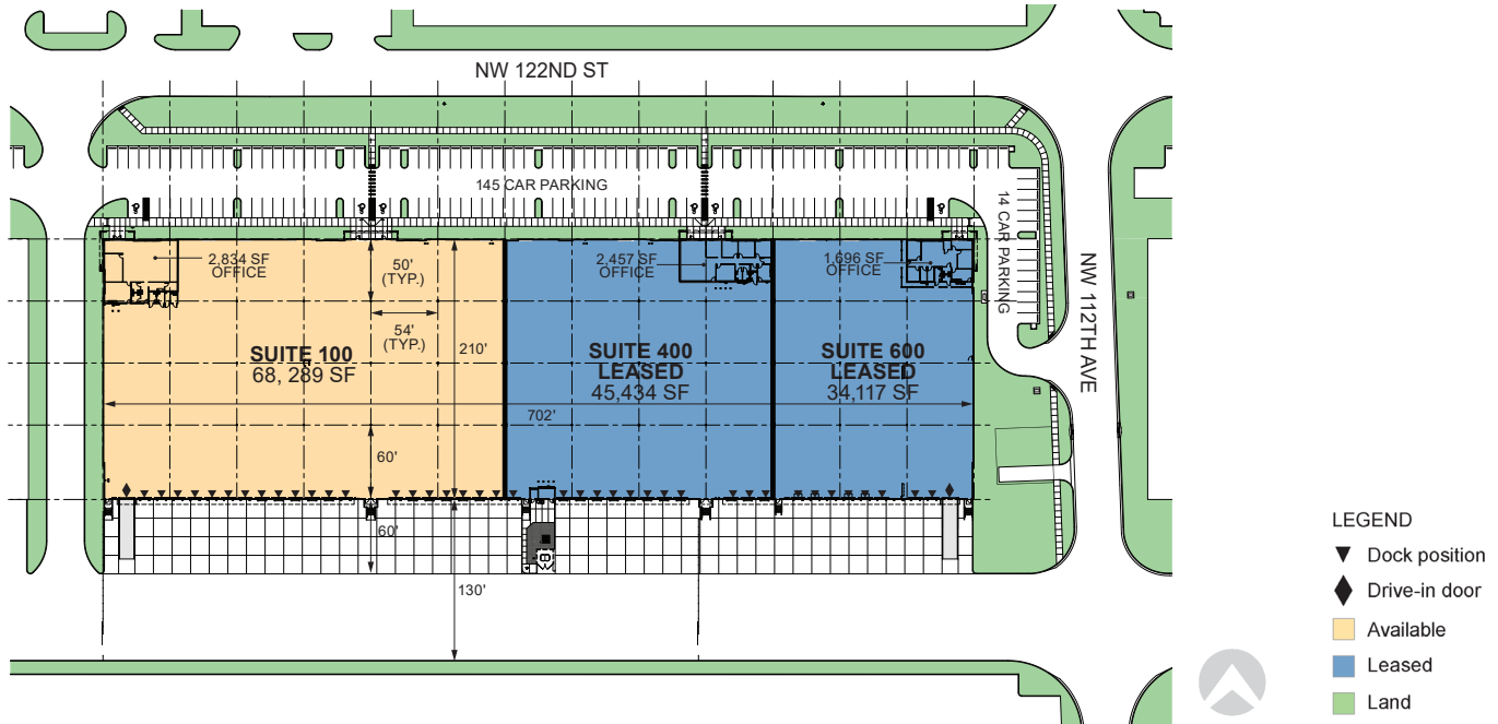
OVERALL AREA PLAN - 68,289 SF
