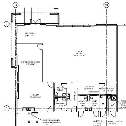
OFFICE SPACE - 2,834 SF
