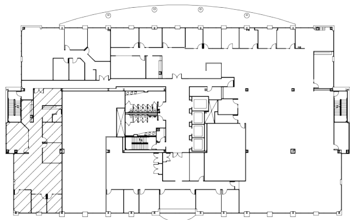
BUILDING KEY PLAN SECOND FLOOR
