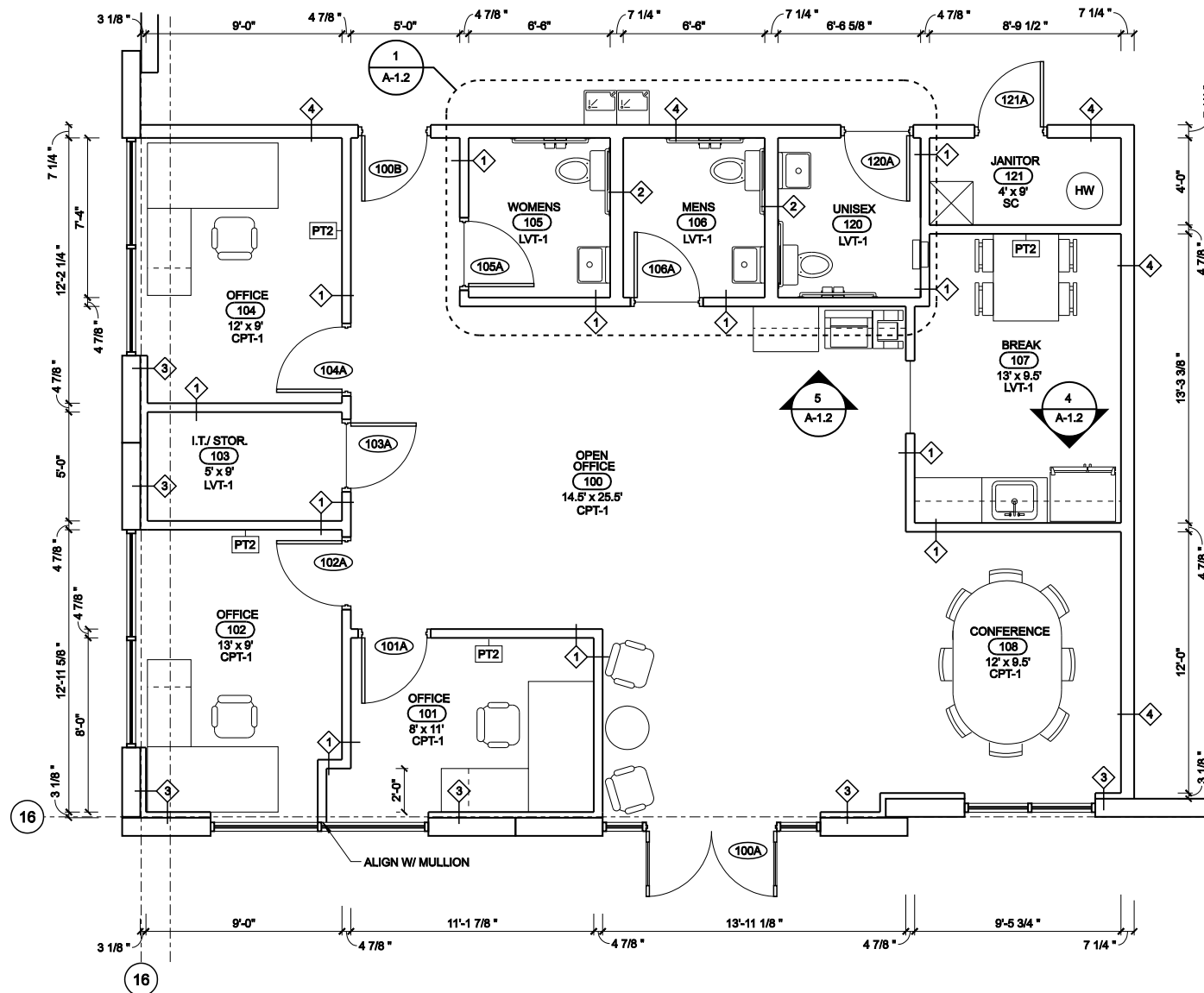
1 ENLARGED FLOOR PLAN SCALE: 1/8" = 1'-0" OFFICE = 1,443 SF
