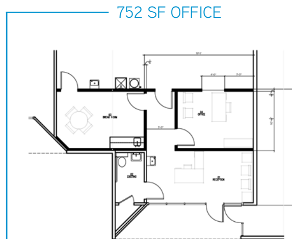
OFFICE PLAN
