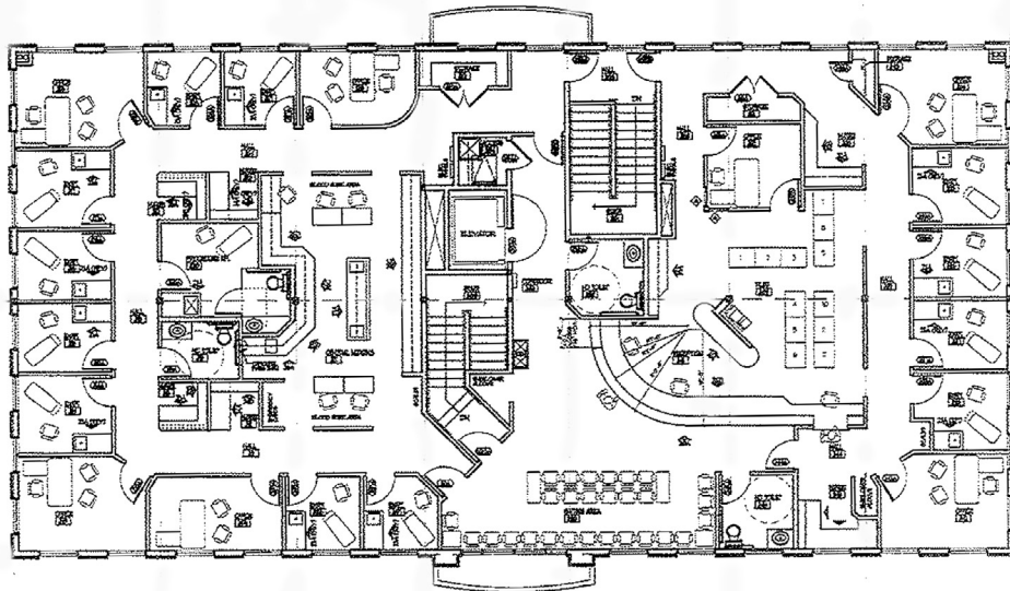
Third Floor
