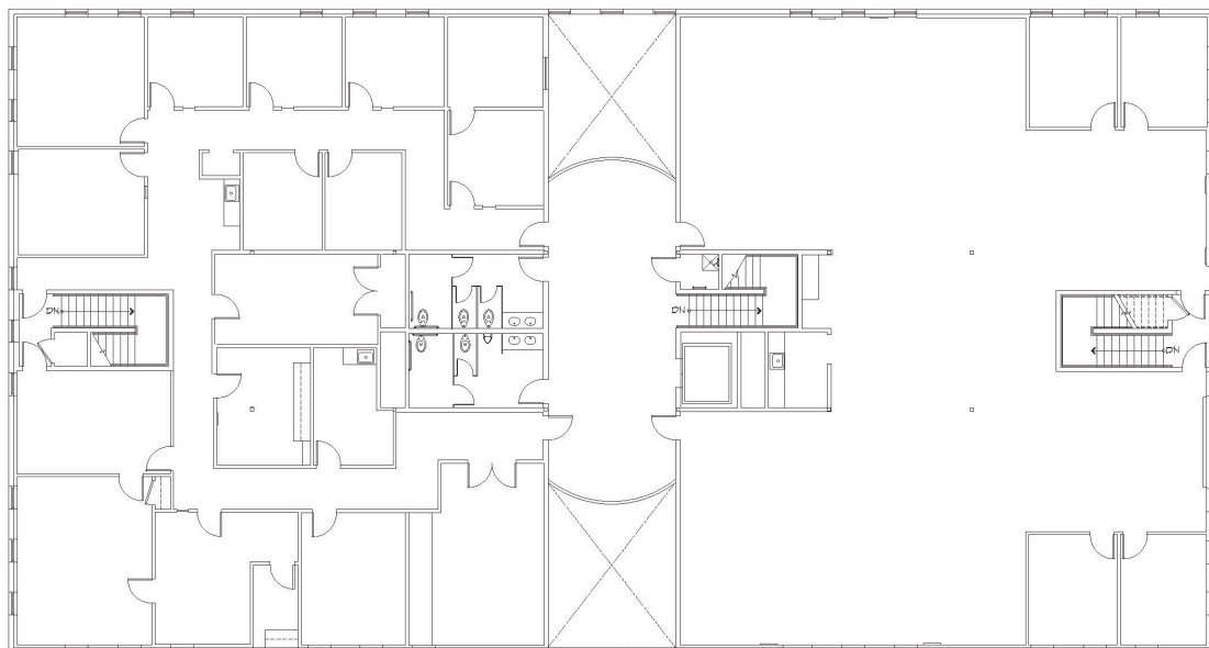
SECOND FLOOR
