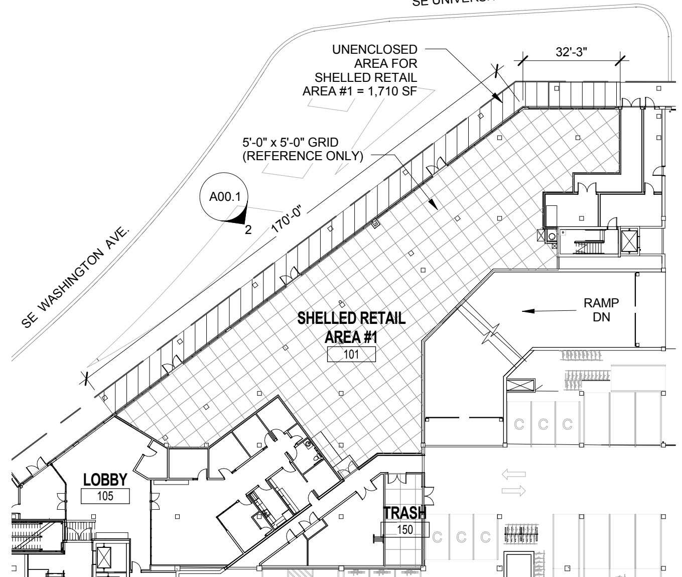
1 A00.1 LEVEL 1 PLAN - RETAIL AREA #1 1/32" = 1'-0"
