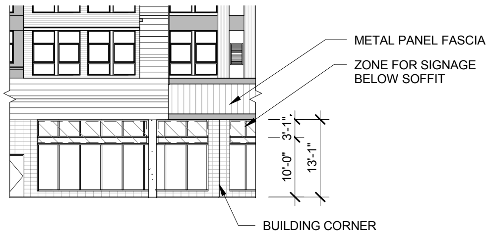
3 A00.1 RETAIL #1 - ELEVATION 2 1/16" = 1'-0"
