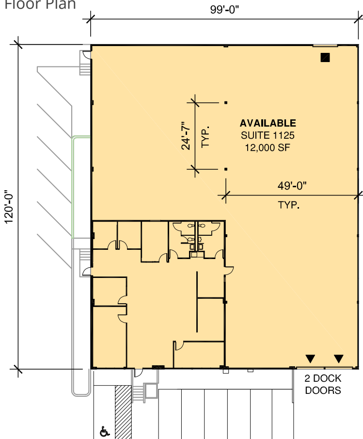
Floor Plan
