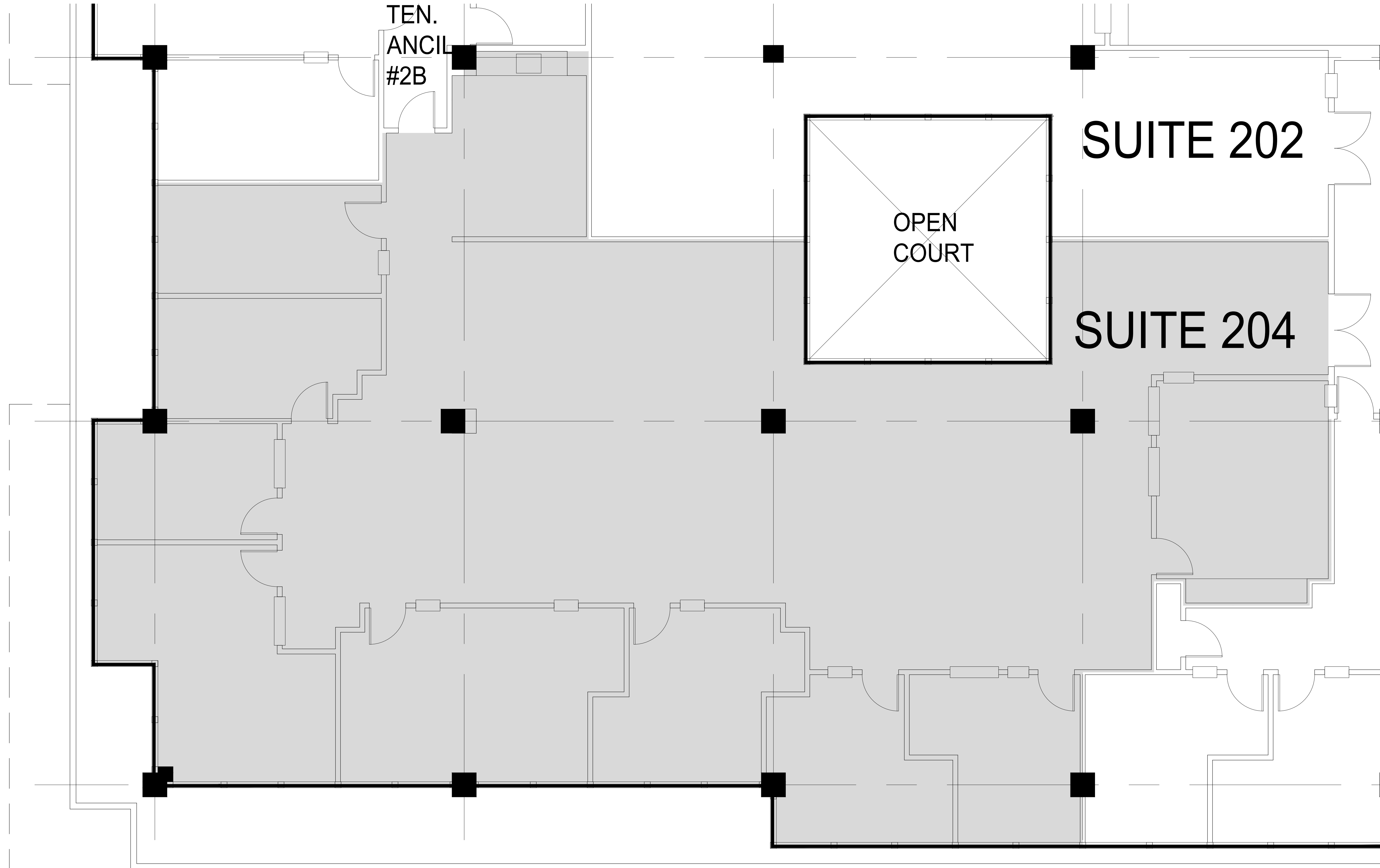
1 FLOOR PLAN - SUITE 204 SCALE: 1/4" = 1'-0"
