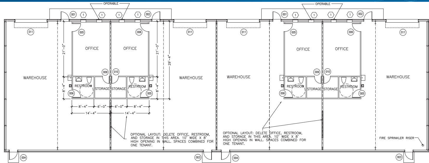
FLOOR PLAN (BUILDING FGHI)
