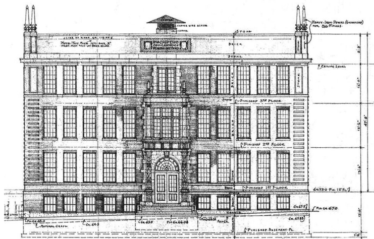
NORTH (EAST 4 TH ST) ELEVATION
