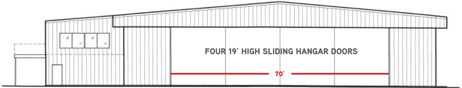
NORTHEAST ELEVATION
