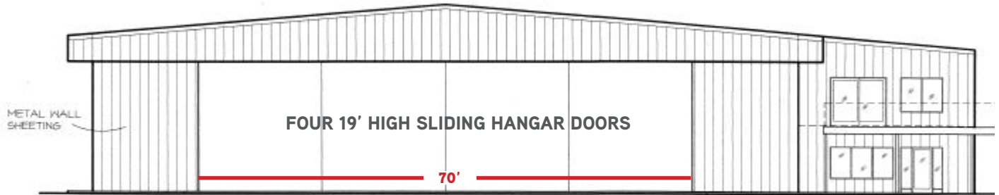
SOUTHWEST ELEVATION
