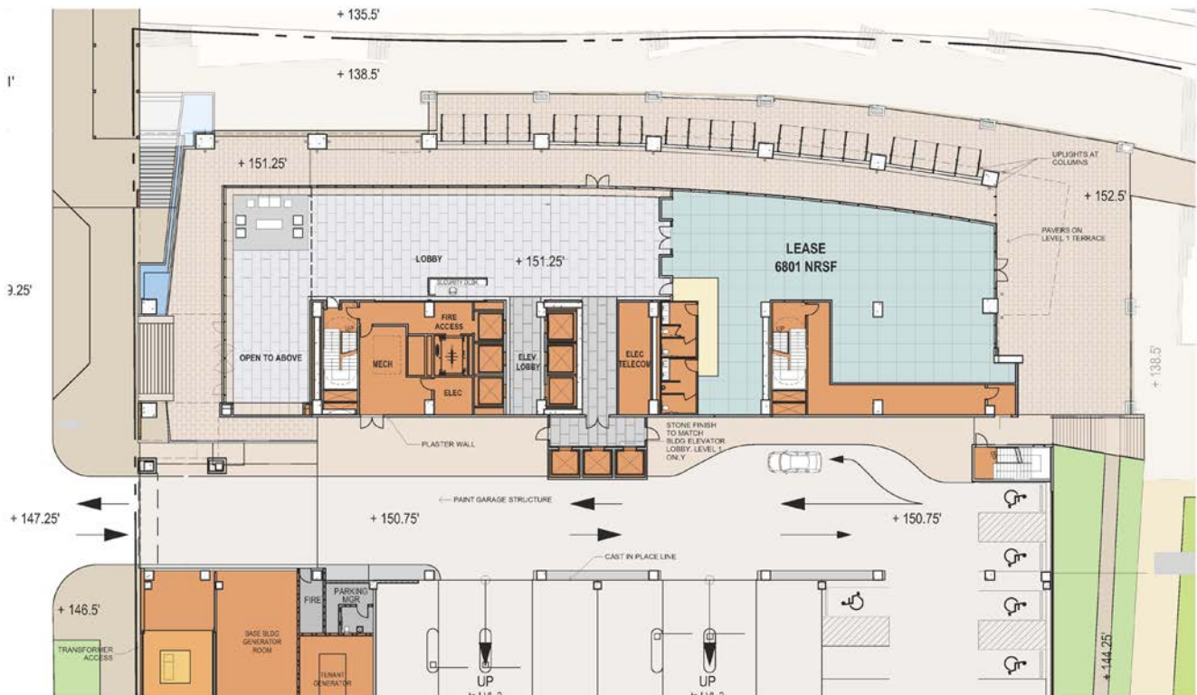
FIRST FLOOR
