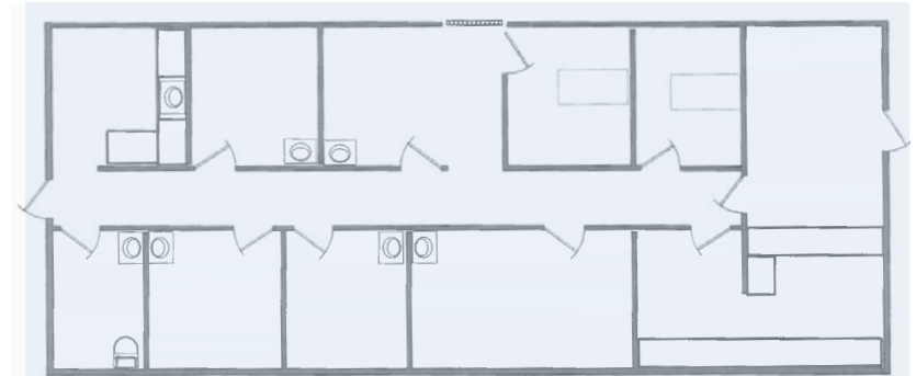
FLOOR PLAN
